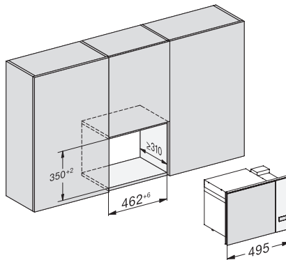
M22xxSC, installation drawing
