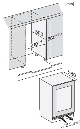
KWTUS7196E, Built-under, installation diagram, niche dimensions
