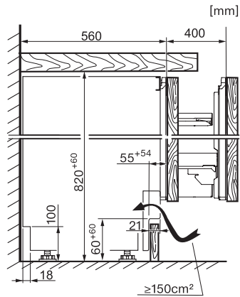
KU7030D, Built-under, side view
