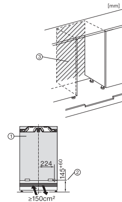
KU7030D, Built-under, installation drawing
