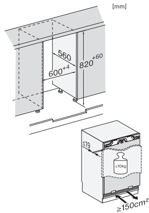
KU7030D, Built-under, installation diagram, niche dimensions
