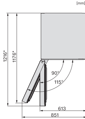
KWNS4784DE edt/cs, Rioja, top view
