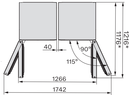
KWNS4784DE edt/cs, Rioja, top view
