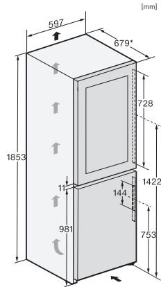
KWNS4784DE edt/cs, Rioja, installation sketch
