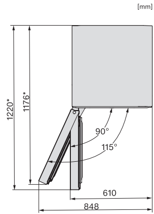
FNS4882D, top view (footnote*) (installation drawings)
