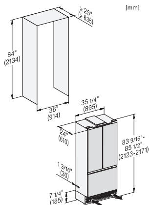
KFMC3642FD, KFMC3844FD, MasterCool III, integration, panel ready (installation drawing) (US)
