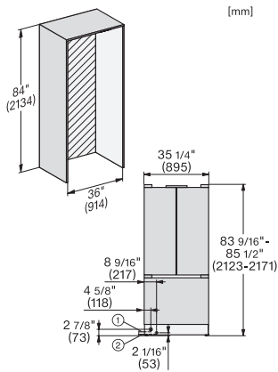
KFMC3642FD, KFMC3844FD, MasterCool III, installation, panel ready (*Footnote) (installation drawing) (US)
