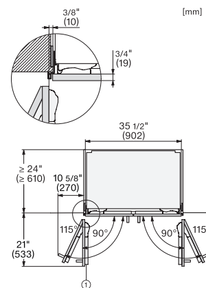
KFMC3642FD, KFMC3844FD, MasterCool III, PACS, with stainless steel front, top view (installation drawing) (US)
