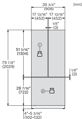
KFMC3642FD, KFMC3844FD, MasterCool III, front view (*Footnote) (installation drawing) (US)
