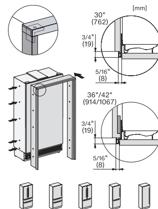
KFMC3632R+L, KFMC3642R+L, KFMC3836R+L, KFMC3834R+L, KFMC3858FD, MasterCool III, frame neutral, installation (drawing)
